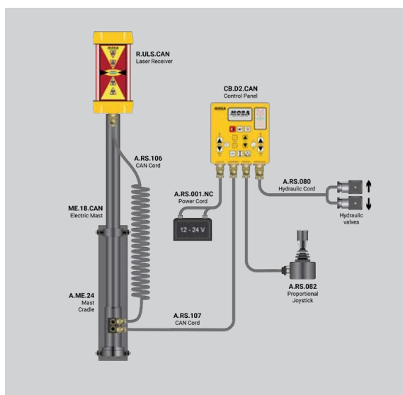
RS.033 Typical single receiving system
